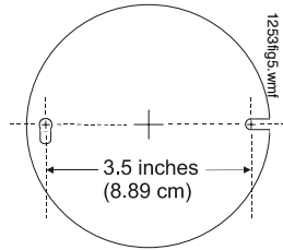
Figure 5 Model 30-2021E-24 Mounting Holes
