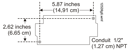
Figure 6 Model 30-2021E-24 Mounting Holes
